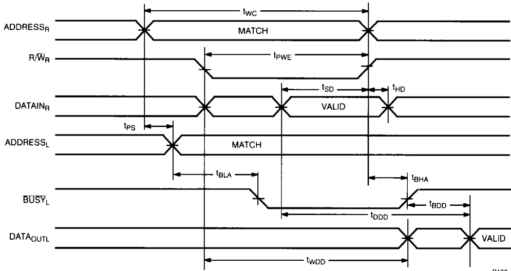
Timing Diagram of Read with \overline{\text{BUSY}} ( M/\overline{S}=\text{HIGH} ) [2]
