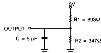
(c) Three-State Delay (Load 3)
